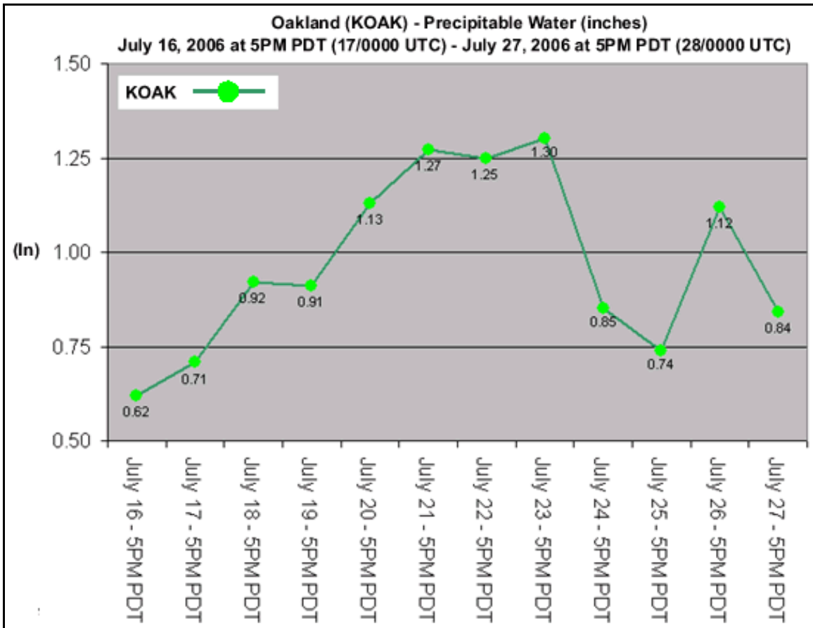
Figure 18: Depicts the precipitable water values (inch) recorded at the Oakland (KOAK) sounding site during the afternoon launches. Notice the increase in monsoonal moisture through the heat wave event, peaking between July 21 and July 23. This correlates well to the elevated overnight minimum temperatures, which peaked on July 23.
