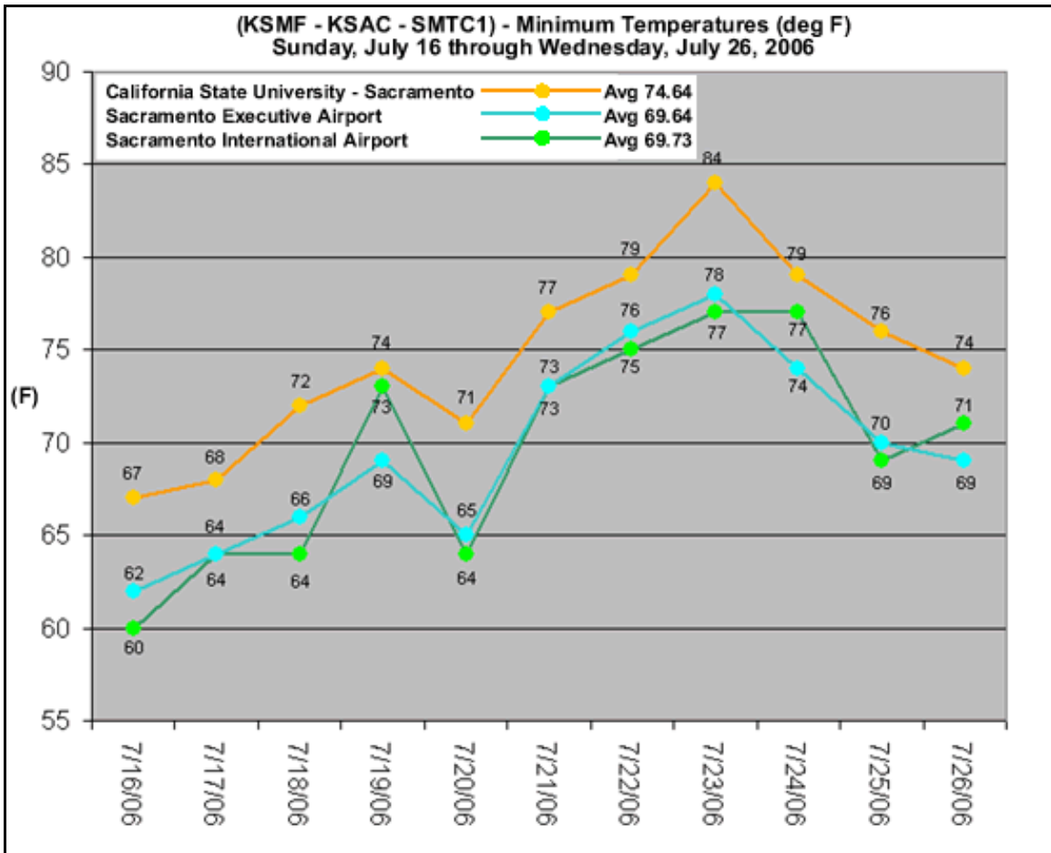
Figure 20: Depicts overnight minimum temperatures at three locations throughout the Sacramento region during the July 2006 heat wave event. All three locations recorded elevated minimum temperatures; however, the urban heat island effect was noted at the California State University – Sacramento observation station. The average temperature was approximately 5°F warmer than the Sacramento International and Executive Airports.
