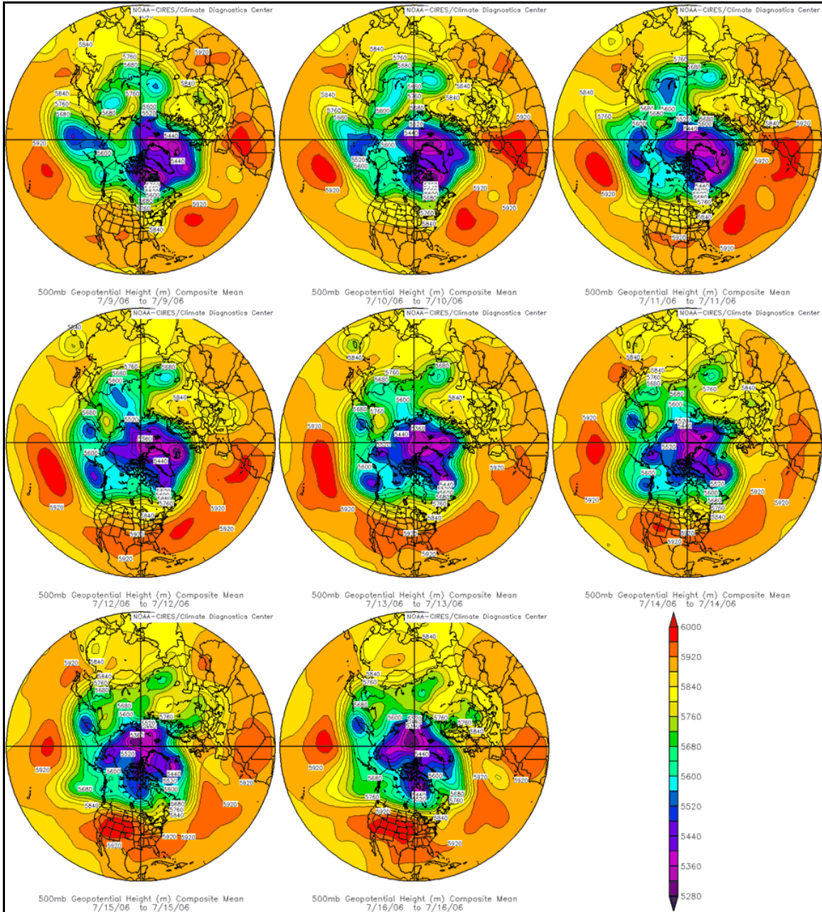
Figure 4: Displays daily averaged 500mb geopotential heights (m) from July 9 through July 16, 2006 (representing the week leading up to the heat wave episode). The feature of note is the upper level trough of low pressure off the eastern Russia coast over the western Pacific. This disturbance propagates across the northern Pacific before splitting near the Alaska Peninsula. A portion of the energy associated with this system dissipates inland over British Columbia, while a secondary piece of energy digs southward and develops an upper level trough of low pressure along 150°W. This not only resulted in the retrogression of the subtropical upper level high pressure, but also generated a downstream adjustment of the westerly flow and the strengthening of the upper level high pressure across the western United States.
