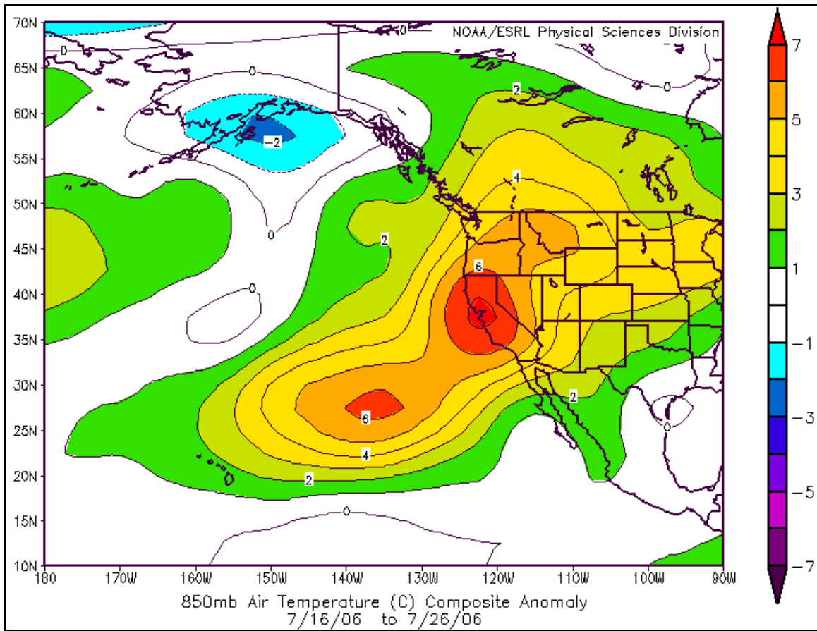
Figure 11: Shows 850mb air temperature (°C) anomalies during the period of the July 2006 heat wave. The strongest anomalies associated with the warm air mass across the southwest United States were located along the west coast. In particular, the peak departures from normal were located over the San Francisco Bay Area, the southern Sacramento Valley, and northern San Joaquin Valley.
