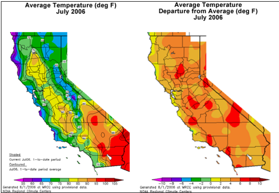
Figure 22: Displays the average temperature (°F) for July 2006, and the departure from normal. As expected, anomalies warmer than normal were recorded across much of the state of California. Peak readings ranged from 6°F to 8°F.
