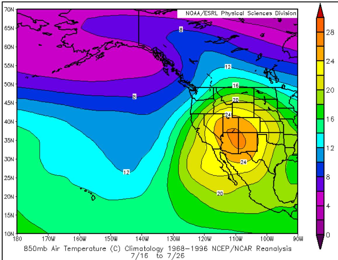
Figure 9: Indicates 850mb air temperature ( ^{\circ}\text{C} ) climatology (1968 – 1996) for the period of the 2006 heat wave (Sunday, July 16 through Wednesday, July 26, 2006). The core of the warm air mass associated with the western United States upper level high pressure ridge is located over the Four Corners region. Across California, typical values rise from near 16^{\circ}\text{C} over northwest California to near 24^{\circ}\text{C} over southeast California.
