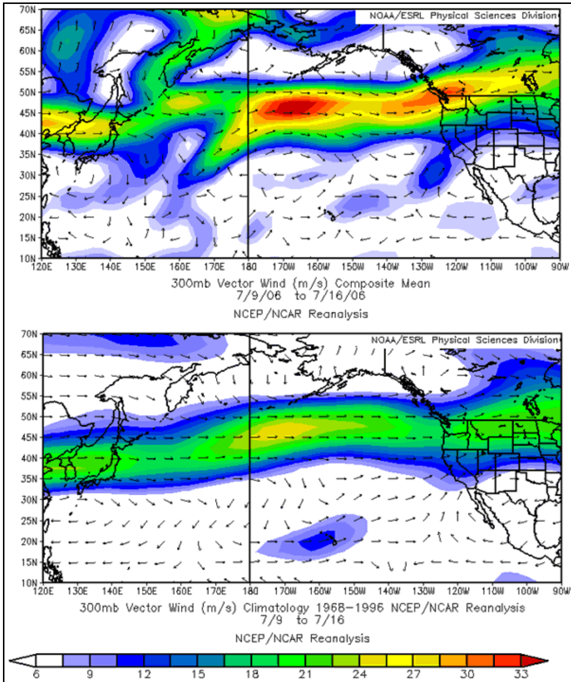
Figure 5: Specifies the 300mb wind speed and vector for the period representing the week prior to the July 2006 heat wave episode (upper graphic), and the climatological mean (1968 – 1996) for the similar time period (lower graphic). Note the enhanced jet stream between 40°N and 50°N due to the increased temperature gradient between the strengthening subtropical high and the cooler troughs traversing the northern Pacific. Also, on the July 9 through July 16, 2006 image, the jet stream indicates a split as it crosses 150°W with vector divergence apparent.
