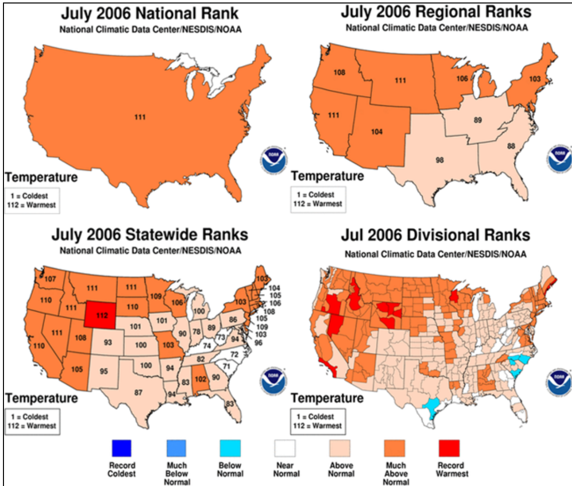
Figure 26: The above graphic shows a breakdown of the July 2006 temperatures, ranking each area based on the past 112 years of observed data. The data is ranked for areas as large as the lower 48 United States down to smaller divisions within each state. The lower 48 United States recorded its second warmest July on record. Looking at California, the state saw its third warmest July. When considering California by climate division, the south coast of California experienced its warmest July ever, while other areas of the state saw either above normal or much above normal conditions.
