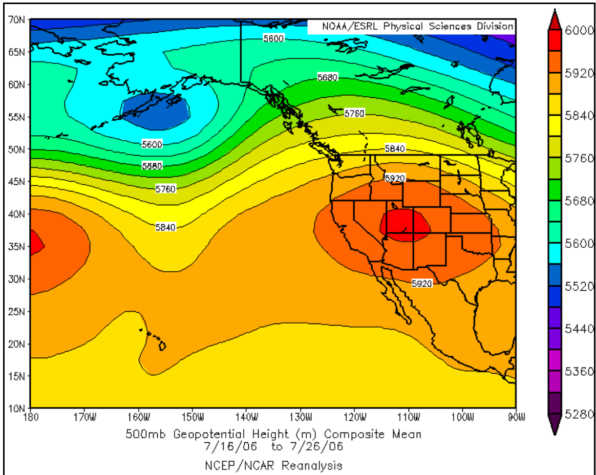
Figure 2: Displays the composite mean of the 500mb geopotential heights (m) through the duration of the July 2006 heat wave. The semi-permanent summertime upper high pressure ridge across the western United States strengthened and displaced westward with its core located over southern Utah. This pattern adjusted flow across much of California with easterly to southerly winds.
