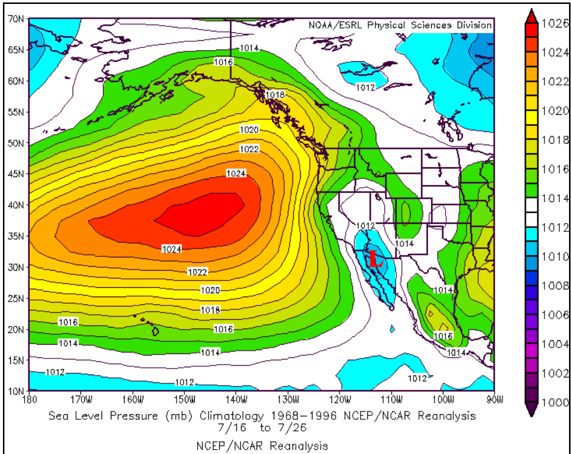
Figure 13: Climatology (1968 – 1996) indicates a thermally induced surface low pressure center located south of Yuma, Arizona over northwest Mexico. A thermal trough extends northward from this surface low, and is generally aligned along the Nevada and Utah border. Also, note a broad area of surface high pressure centered over the eastern Pacific Ocean. This generates northwesterly surface flow over coastal waters of the western United States, as well as upwelling of cooler waters in the same region.
