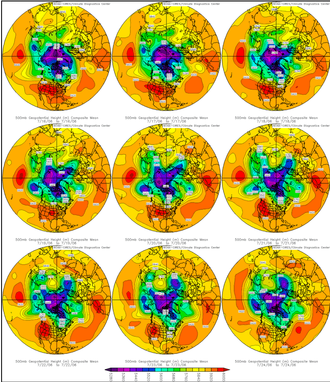
Figure 6: Displays daily averaged 500mb geopotential heights (m) from July 16 through July 24, 2006. This represents the majority of the heat wave, including the peak of this event occurring between Friday, July 21 and Monday, July 24, 2006. The feature of note is another upper level short wave trough of low pressure over the Kamchatka Peninsula of eastern Russia on July 16. This system propagated eastward over the northern Pacific Ocean over the next 3 to 4 days before deepening between 150°W and 160°W. This strengthening upper level trough of low pressure over the east-central Pacific Ocean resulted in prolonging the heat wave episode, and reinforcing the already anomalous western United States upper level ridge of high pressure ridge.
