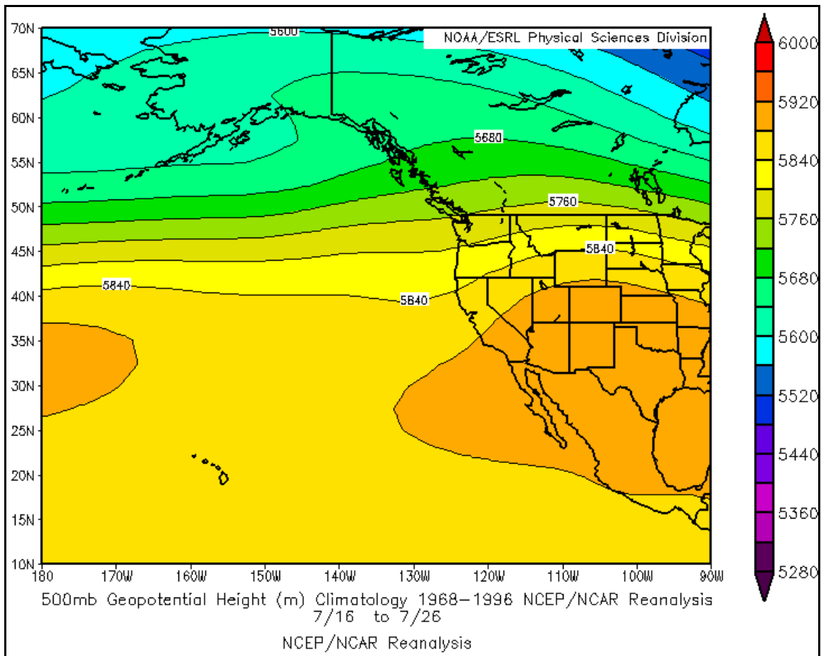
Figure 1: Indicates 500mb geopotential height (m) climatology (1968 – 1996) for the period of the 2006 heat wave (Sunday, July 16 through Wednesday, July 26, 2006). Weak upper level ridging is generally aligned along the crest of the Rocky Mountains with a center over the state of New Mexico. Dry west to southwest flow is situated along the west coast of the United States.
