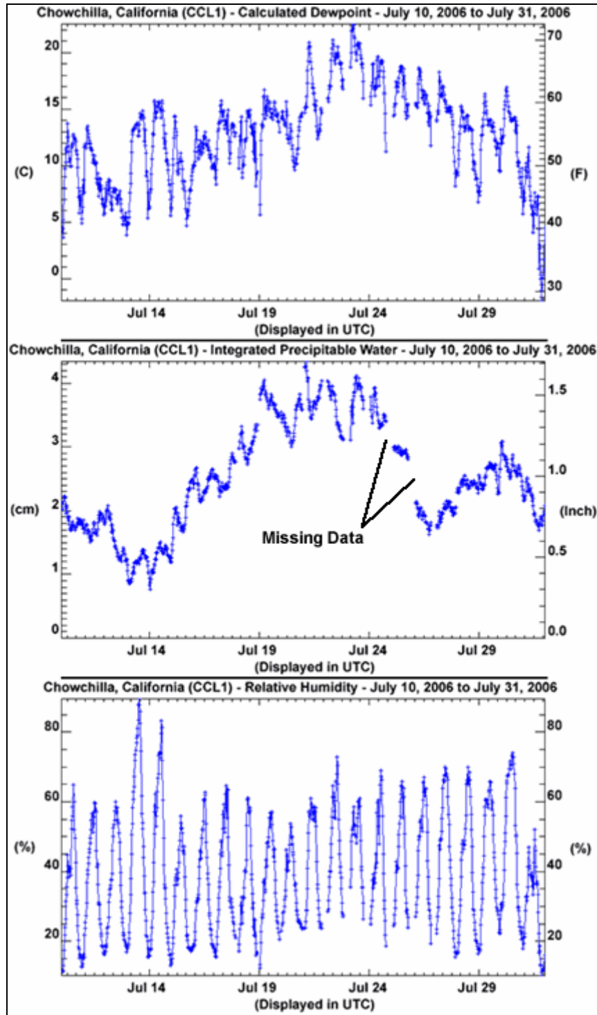
Figure 16: Depicts three unique moisture parameters, surface dew point temperature, integrated precipitable water, and relative humidity at Chowchilla, California (north-central San Joaquin Valley) from July 10 through July 31. Notice the increase of surface dew point temperature and integrated precipitable water values during the peak of the heat wave event. Also, notice the lack of change in relative humidity, except for typical diurnal fluctuations.
