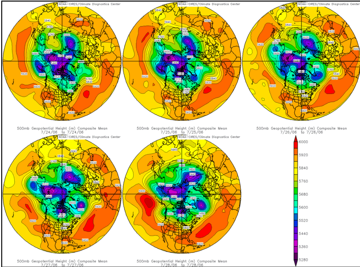
Figure 8: Displays daily averaged 500mb geopotential heights (m) from July 24 through July 28, 2006. This represents the dissipating phase of the heat wave event where flow transitioned from an easterly to southerly regime to a more climatologically dry west to southwest flow. Note the weakening of both the subtropical upper level high pressure ridge centered near the International Date Line and western United States upper level high pressure ridge. In the last couple frames, a deep upper level low pressure trough developed over the western Pacific, resulting in the expansion of the subtropical upper level high pressure ridge north of Hawaii. Given this pattern shift, a system over the Gulf of Alaska dropped southeast, turning flow over the west coast of the United States to a climatologically dry west to southwest.
