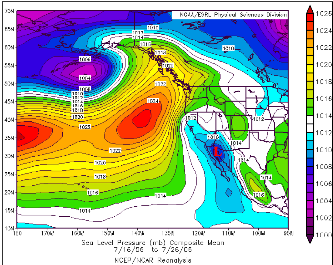
Figure 14: Displays sea level pressure (mb) during the July 2006 heat wave episode. The position of the thermally induced surface low and the alignment of the weak thermal surface low along the Nevada and Utah border are similar to climatology. However, a deeper thermal surface trough developed along the west coast of California. This thermally induced surface trough allowed for onshore westerly winds to shift to an easterly direction with lowered magnitudes. The marine layer along the coast, which typically penetrates inland during the overnight hours, was kept along the immediate coast. Also, the typical northwesterly pressure gradient along the coast of California was much weaker, resulting in calmer winds at buoys and a reduction of the upwelling of cooler ocean waters.
