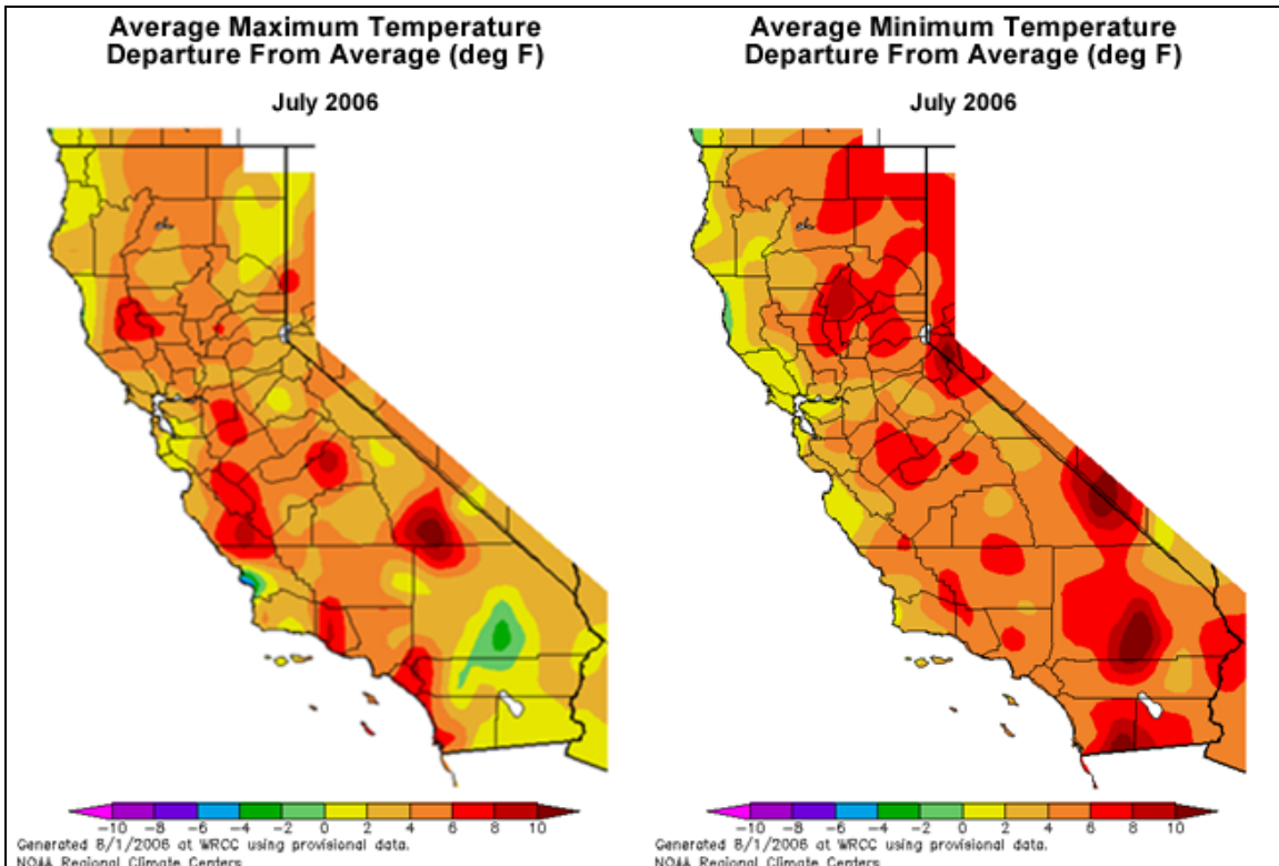
Figure 21: Depicts the departure from average for both the average maximum and average minimum temperature ( ^{\circ}\text{F} ) for July 2006. As one would expect, average maximum and average minimum temperature both exhibited above normal conditions across much of California. In fact, one of the aspects that made the July 2006 heat wave noteworthy was the elevated overnight minimum temperatures, which is reflected well in the right hand image.
