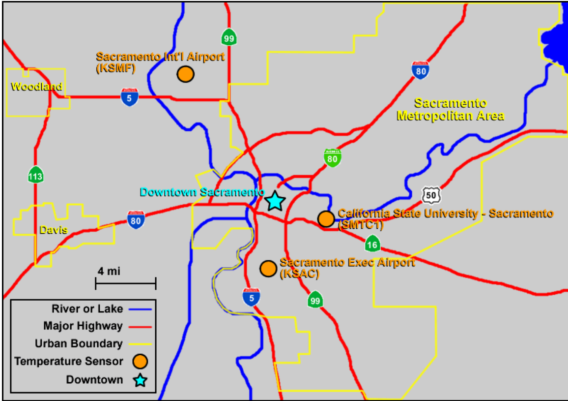
Figure 19: Displays the three observation stations located throughout the Sacramento region. Also, the general urban boundary is depicted. Sacramento International Airport is in a rural setting just outside the urban boundary to the northwest. Sacramento Executive Airport is located near the edge of the urban boundary on the southwest part of the area. California State University – Sacramento is located near the middle of the Sacramento urban area.
