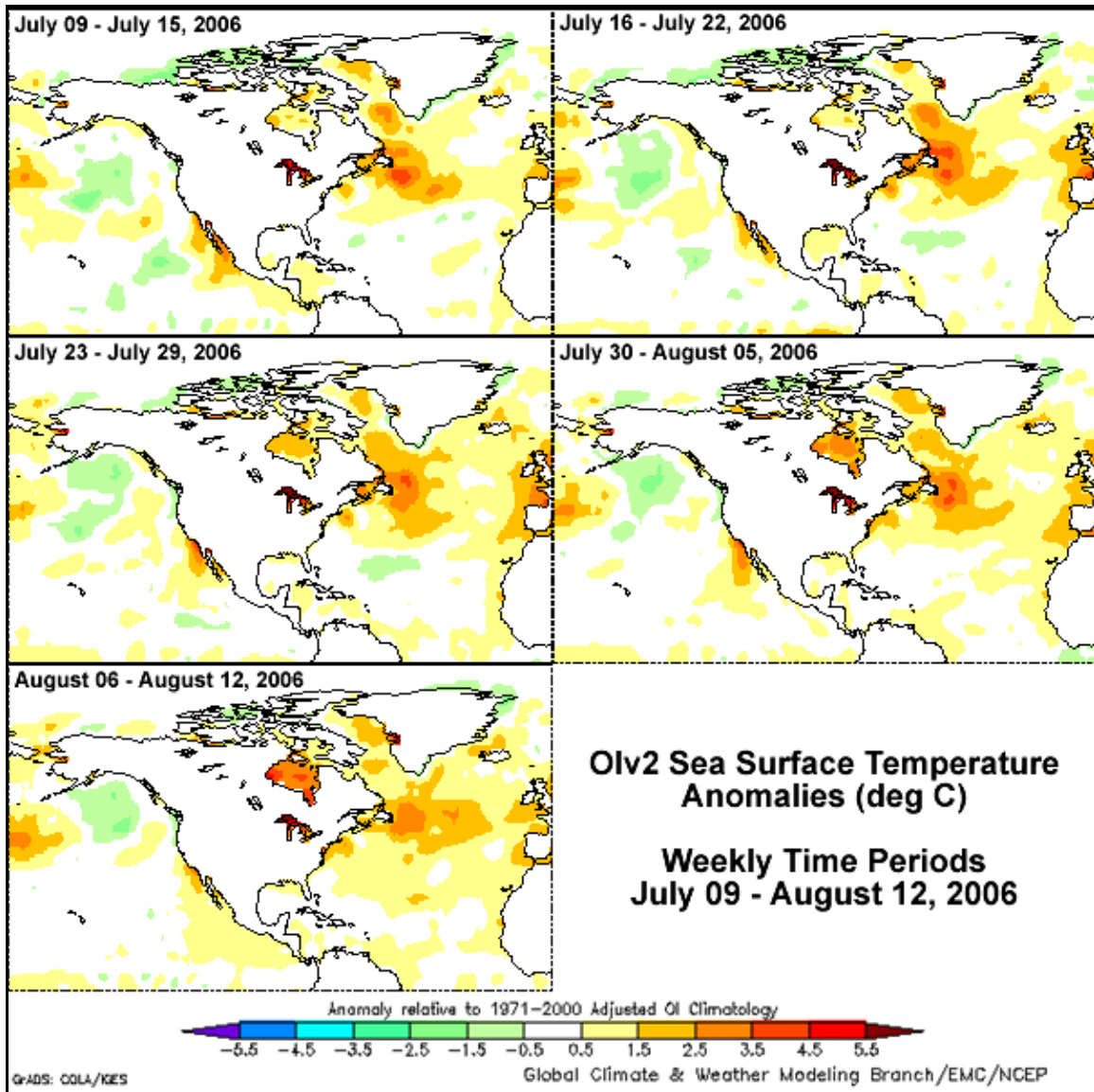
Figure 15: Represents weekly sea surface temperature anomalies for the period of July 9 through August 12, 2006. Note the increase in positive anomalies along the California coast from San Francisco to the United States and Mexico border during the heat wave event, peaking between July 23 and August 5, 2006. This increase in sea surface temperatures was the direct result of the weakening northwesterly gradient along the California coast, which resulting in a reduction of upwelling of cooler ocean waters. Finally, as the northwesterly gradient returned in August 2006, a lessening of the anomalies is noted in the week of August 6 through August 12.
