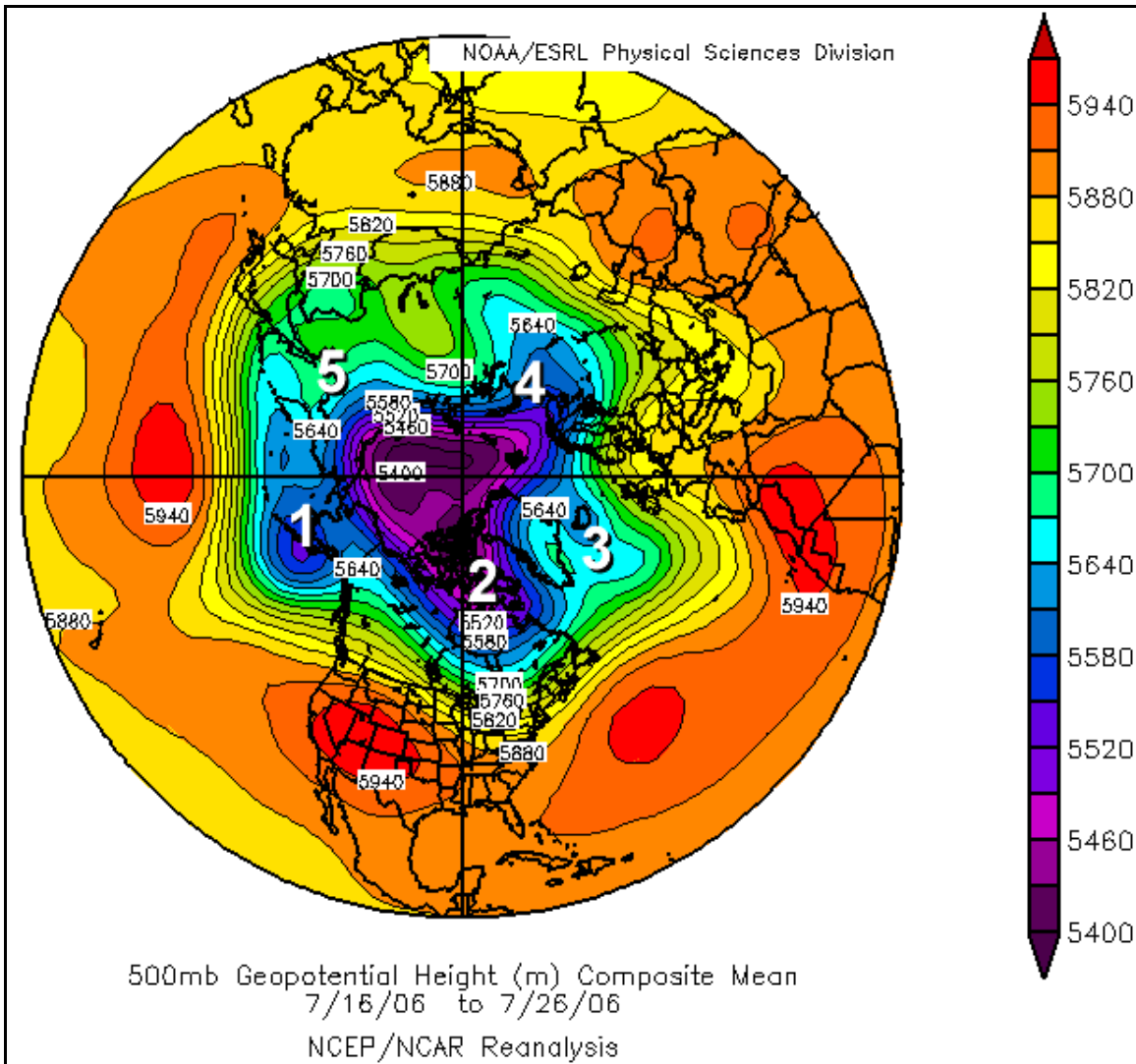
Figure 3: Shows the northern hemispheric 500mb geopotential height (m) composite mean throughout the heat wave episode. The building upper high pressure ridge responsible for the state of California heat wave centered over southern Utah was part of an overall amplification of the flow across the entire northern hemisphere, which resembled a wavenumber 5 pattern (albeit weak given the summer season). Please note the annotated numbers in large white numbers (1 through 5) indicating the waves.
