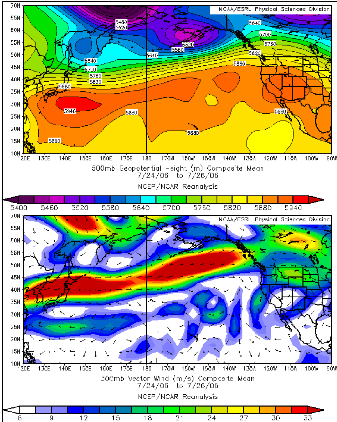
Figure 7: Indicates the 500mb geopotential heights (m) and 300mb vector wind (m/s) from July 24 through July 26, 2006. This shows the increasing heights across the east-central Pacific, as well as the strengthening zonal jet stream crossing the Pacific. This zonal jet stream reduced the amplified flow, including the western United States upper level high pressure ridge responsible for the July 2006 heat wave.
