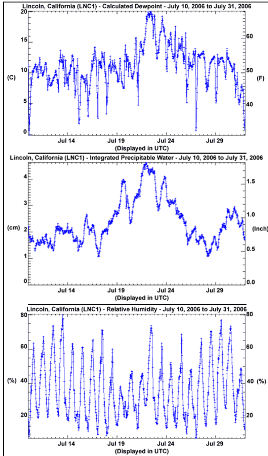
Figure 17: Depicts three unique moisture parameters, surface dew point temperature, integrated precipitable water, and relative humidity at Lincoln, California (southern Sacramento Valley) from July 10 through July 31. Notice the increase of surface dew point temperature and integrated precipitable water values during the peak of the heat wave event. Also, notice the lack of change in relative humidity, except for typical diurnal fluctuations.
