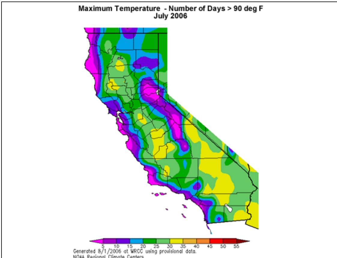
Figure 23: This graphic displays the number of days the maximum temperature was above 90°F. As expected, the greatest numbers were located across the Sacramento Valley and San Joaquin Valley, as well as the interior deserts of southeast California.
