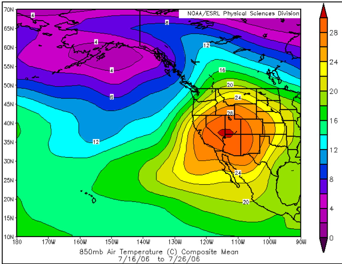
Figure 10: Displays the composite mean of 850mb air temperatures (°C) through the duration of the July 2006 heat wave. The core of the warmest air across the southwest United States shifted westward over southern Nevada and southwest Utah. The typical warm air mass over the southwest United States expanded and encompassed a bigger area.
