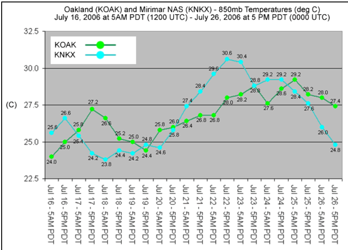
Figure 12: Indicates 850mb temperatures (°C) recorded at the Oakland (KOAK) and Miramar Naval Air Station (KNKX) sounding locations. Of note is the early peak of warm temperatures at both stations, followed by a slight decrease over the next couple days. Late on July 19 or early on July 20, 850mb temperatures rebounded and elevated to extremely warm levels. These temperatures cooled as the result of the weakening of the western United States upper level high pressure ridge and the return of dry west to southwest flow.
