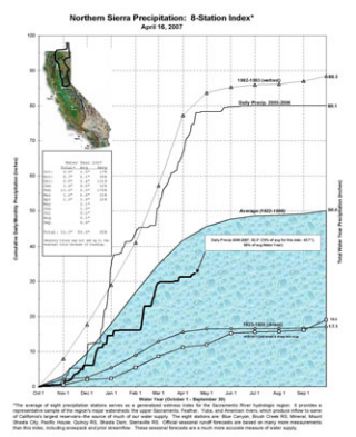
Northern Sierra Precipitation: 8 Station Index
