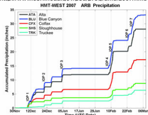
Time series of accumulated precipitation from sensors in the American River Basin during the HMT-West 2007
