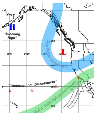
Schematic depicting the general weather pattern over Southern California Jan 7-11, 2005
