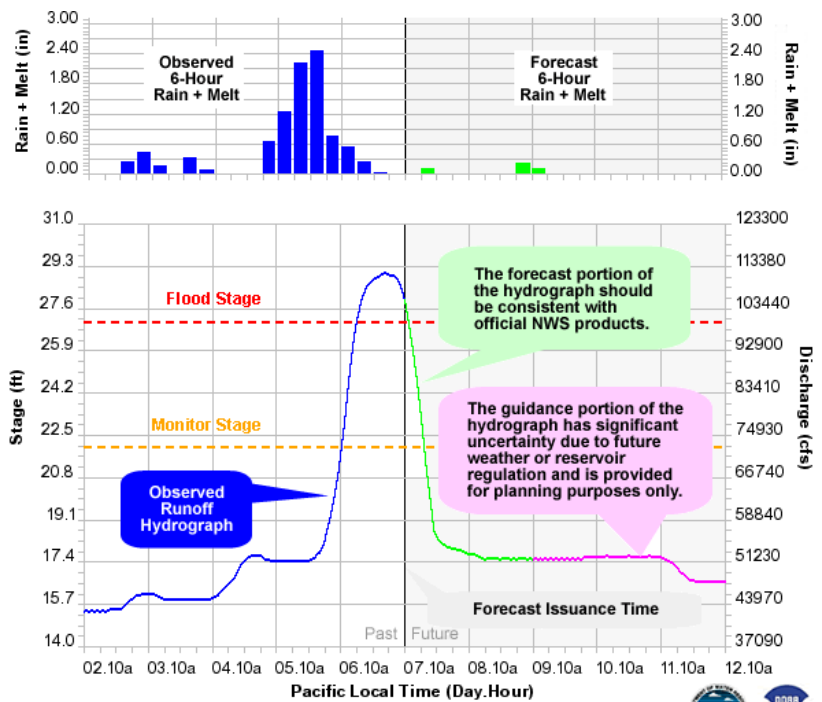
Observed — Forecast — Guidance — Generated 09/07/2005 at 10:15 AM PDT California Department of Water Resources NWS / California Nevada River Forecast Center
